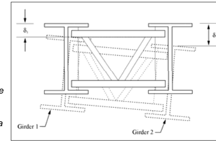
Superstructure cross-section showing steel I-girders and a cross-frame
