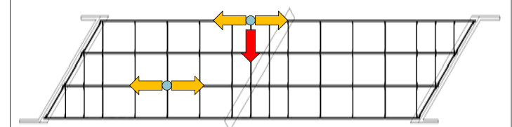
Plan view of a framing plan for a skewed, straight steel I-girder bridge
