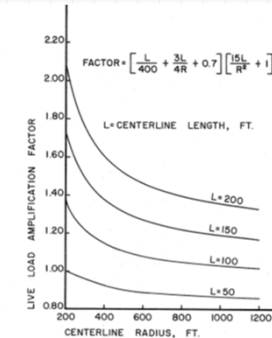
FIGURE 44 AMPLIFICATION FACTOR FOR LIVE LOAD BENDING MOMENT IN THE LONGEST CURVED GIRDER
