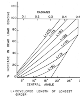
FIGURE 43 PERCENT INCREASE IN DEAD LOAD BENDING MOMENT IN LONGEST CURVED GIRDER
