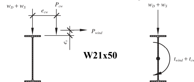
Fig. 6-11. Vertical and torsional loads on spandrel beam.
