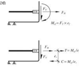
Analysis model for plate design.
