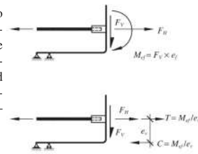
Fig. 5-34. Analysis model for plate design.
